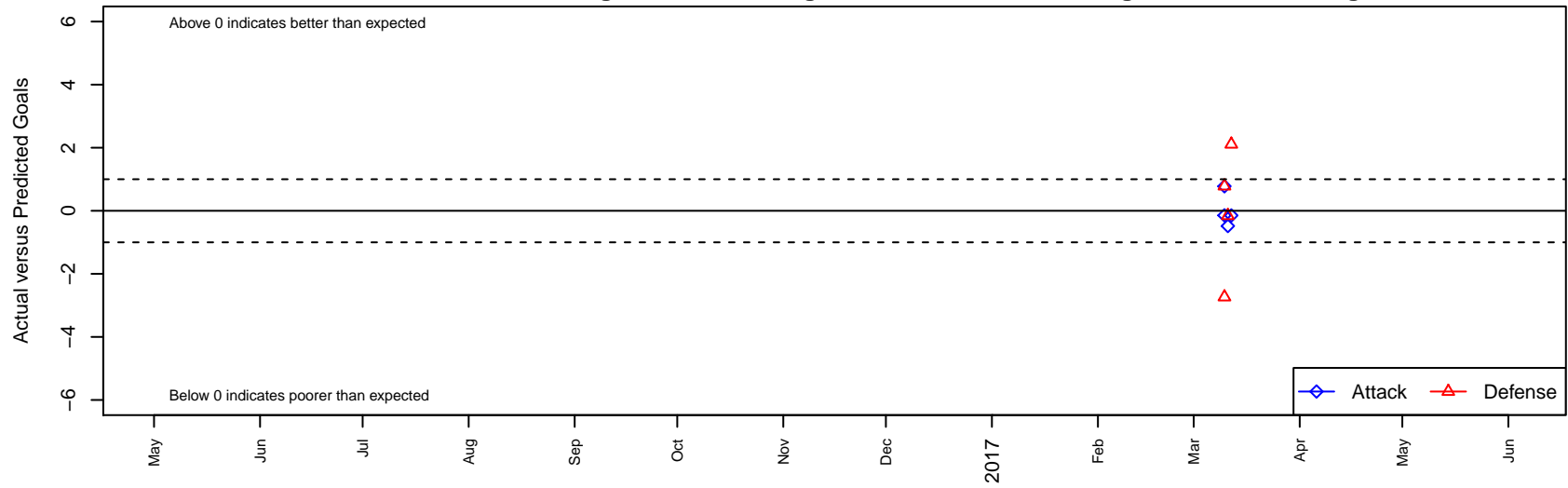
Arsenal Colorado Academy B01 Dots are actual minus expected GF (blue circles) and GA (red triangles). Blue line is smoothed change in attack strength. Red is smoothed change in defense strength.
